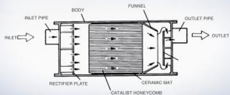
HONEYCOMB TYPE
